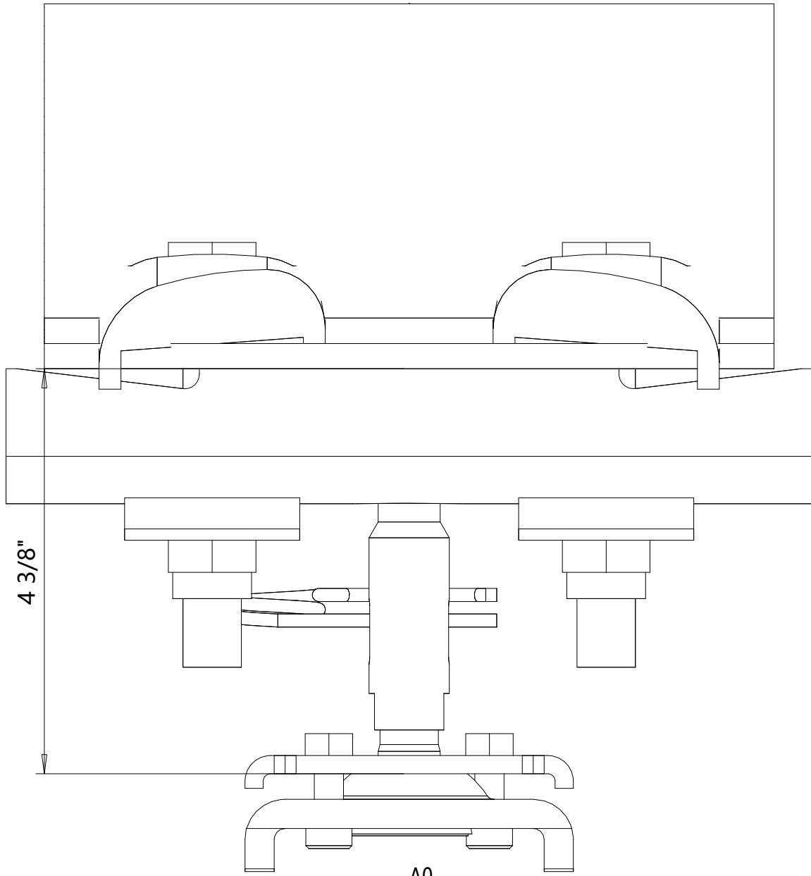
A0 Upper susp. bracket A suits for FLANGE WIDTHS 2 13/16" - 5 1/2"
